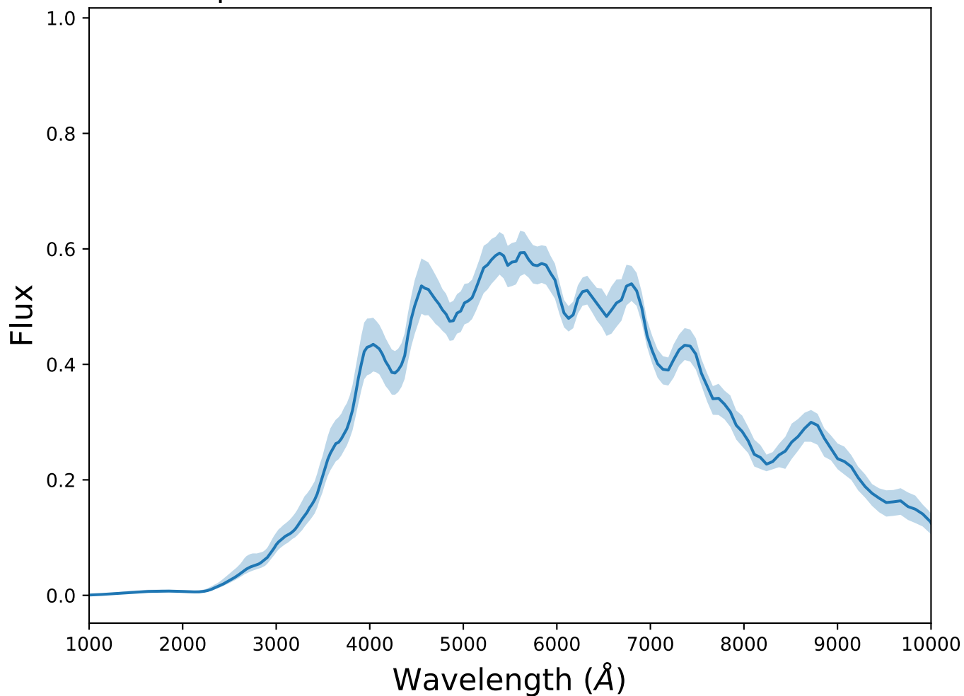
Spectrum 9 for transient SNIax at z=1.06
